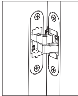
Height Adjustment: Use an allen key to twist the screw (arrow marked) height adjustment: ±1.5mm
