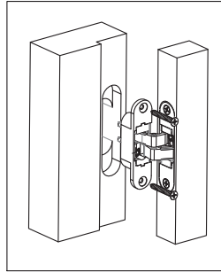
2. Install hinge on the door frame
