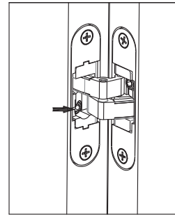
Side Adjustment: Use an allen key to twist the screw (arrow marked) side adjustment: ±1.0mm
