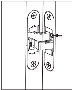
Depth Adjustment: Use an allen key to twist the screw (arrow marked) depth adjustment: ±1.0mm
