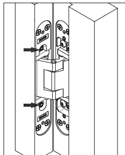
Side Adjustment: -Use an allen key to twist the screws (arrow marked). -Both the upper and the lower screws are requested to be adjusted in the same way. -side adjustment: ±3.0mm
