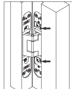
Depth Adjustment: -Use an allen key to twist the screws (arrow marked). -Both the upper and the lower screws are requested to be adjusted and tightened in the same way. -depth adjustment: ±1.0mm
