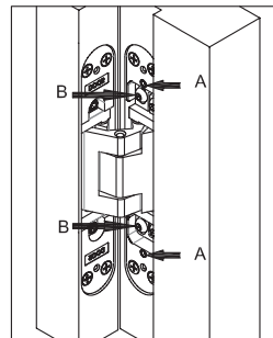
Height Adjustment: -Slightly loosen the grab screws (arrow marked with A) -Use an allen key to twist the screws (arrow marked with B). -Both the upper and the lower screws (arrow marked with B) are requested to be adjusted and tightened in the same way. -Retighten the grab screws (arrow marked with A) -height adjustment: ±3.0mm
